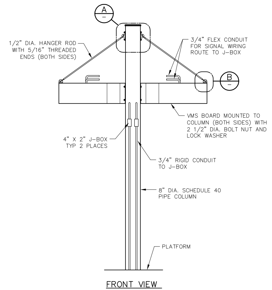
VMS BOARD - COLUMN MOUNT
