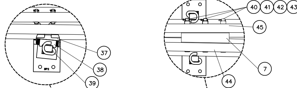
TYPICAL BOLTLESS BRACE ASSEMBLY
