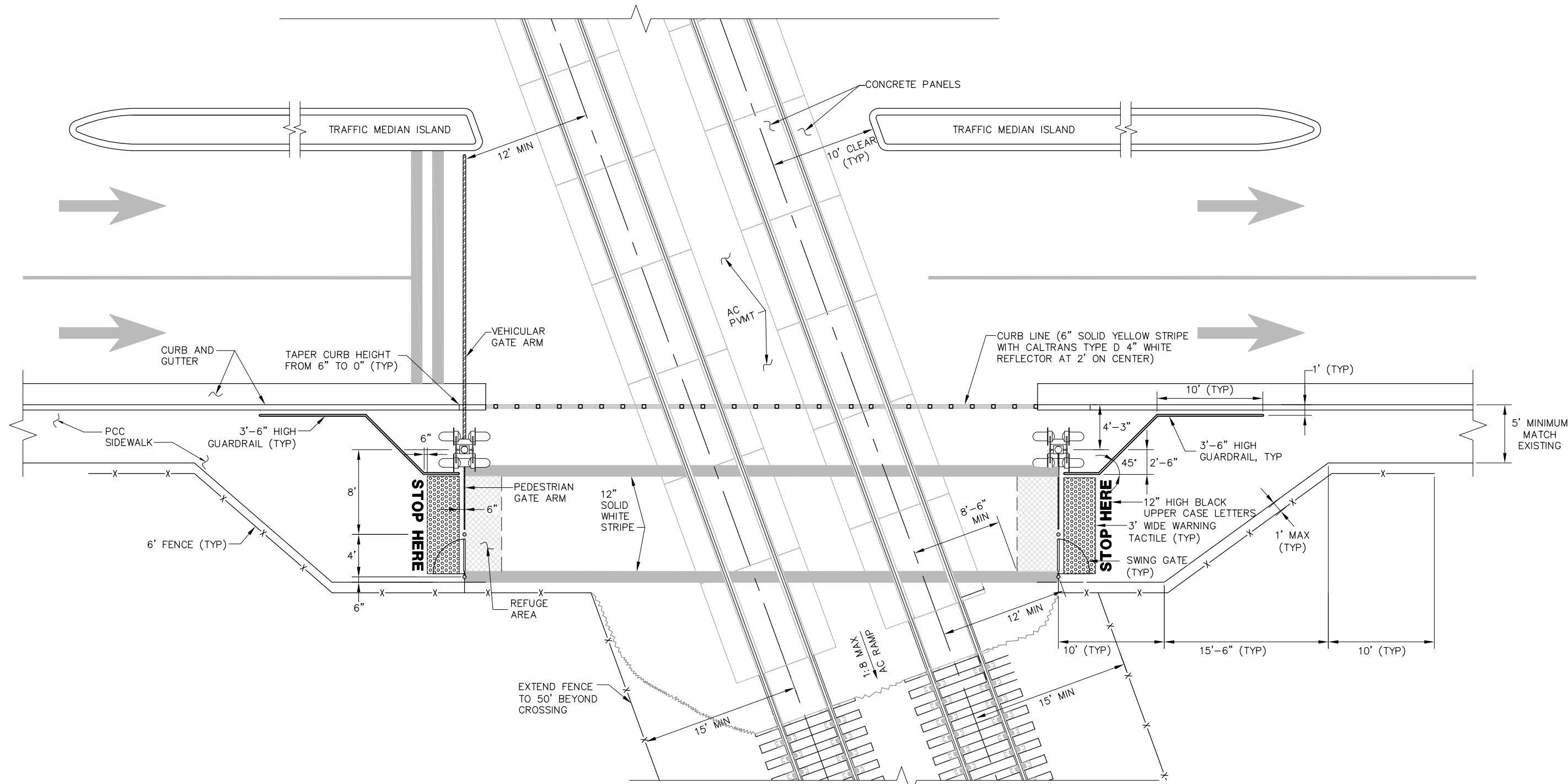
PEDESTRIAN SIDEWALK AT VEHICULAR CROSSING OBTUSE ANGLE INTERSECTION (OPPOSITE END IDENTICAL)
