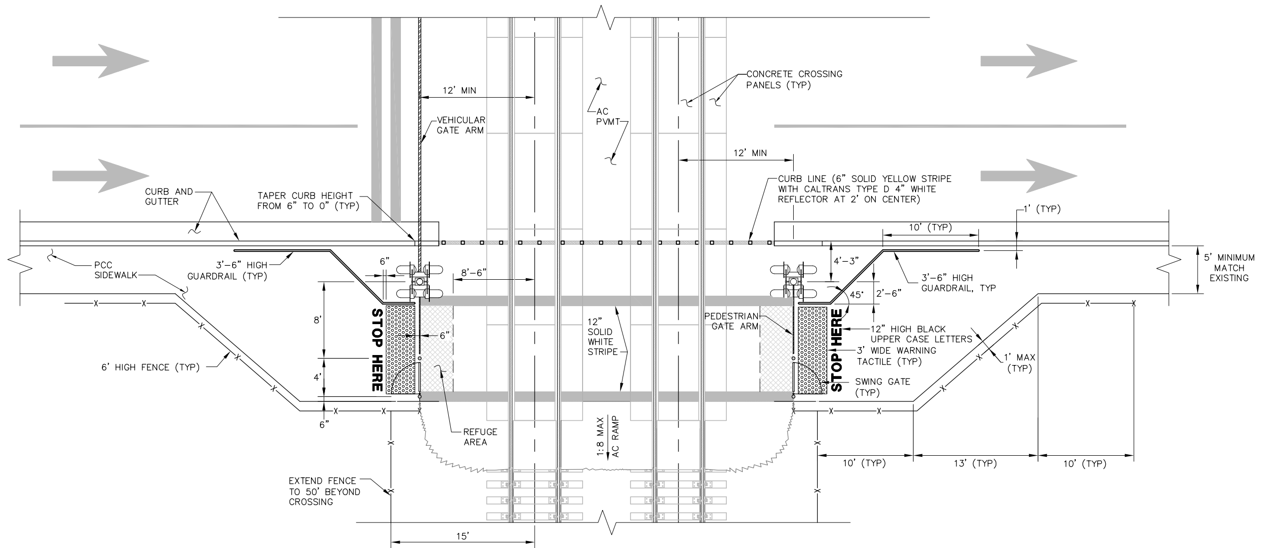
PEDESTRIAN SIDEWALK AT VEHICULAR CROSSING RIGHT ANGLE INTERSECTION (OPPOSITE END IDENTICAL)
